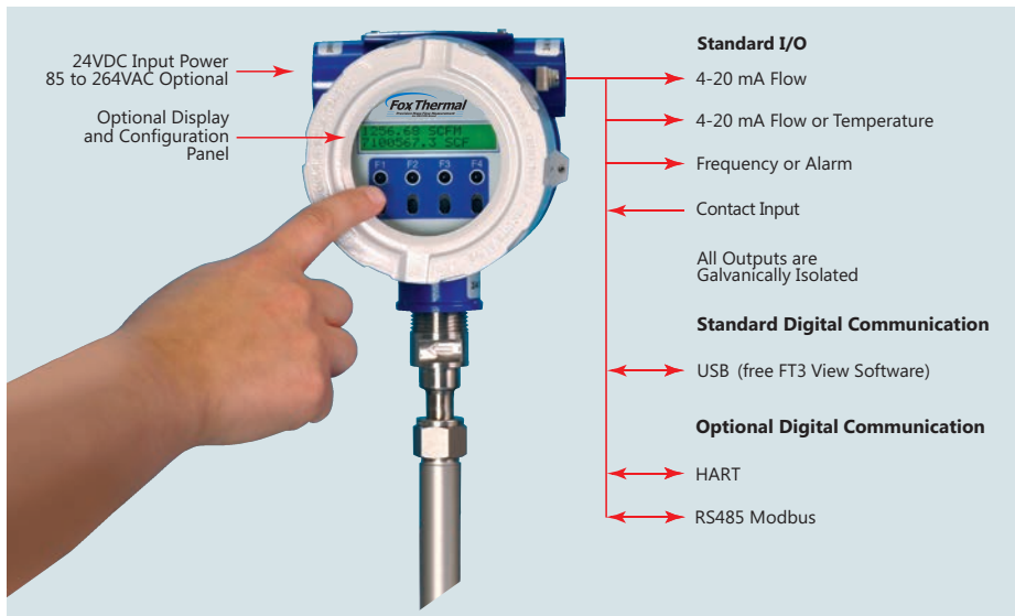
The Model FT3 is a full-featured thermal mass flow meter with a configuration panel that comes equipped with IR buttons for easy configuration of the meter's settings.
